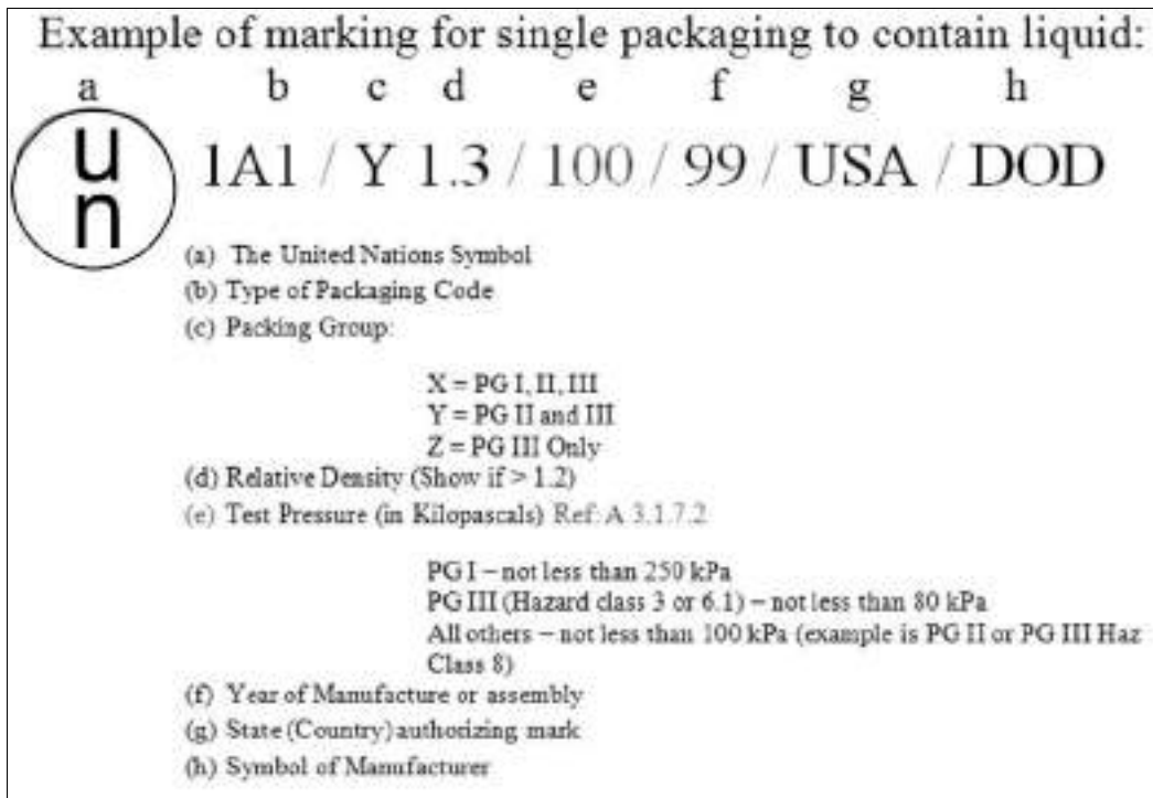
Figure A14.2. Sample of UN Non-bulk Specification Packaging Marking for Liquids.
