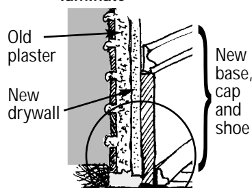
New base over drywall laminate
